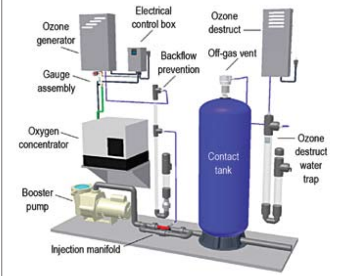
Figure 6. Ozone system components
